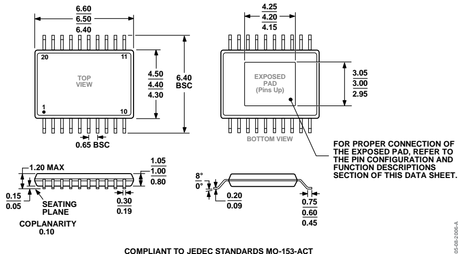
Figure 53. 20-Lead Thin Shrink Small Outline With Exposed Pad [TSSOP_EP] (RE-20-1)
