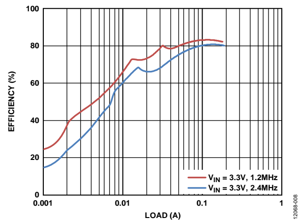
Figure 9. Inverting Regulator Efficiency vs. Current Load, V_{IN} = 3.3 V, V_{NEG} = -5 V, T_A = 25^\circ\text{C}
