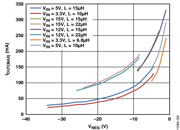
Figure 7. Inverting Regulator Maximum Output Current, f_{SW} = 1.2 MHz, T_A = 25^\circ\text{C} , Based on Target of 70% I_{LIM(INVERTER)}
