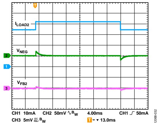
Figure 33. Inverting Regulator Load Transient, V_{IN} = 5 V Step, V_{NEG} = -15 V, I_{LOAD2} = 35 mA to 45 mA Step, f_{SW} = 2.4 MHz, T_A = 25^\circ\text{C}
