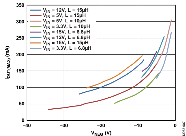
Figure 8. Inverting Regulator Maximum Output Current, f_{SW} = 2.4 MHz, T_A = 25^\circ\text{C} , Based on Target of 70% I_{LIM(INVERTER)}
