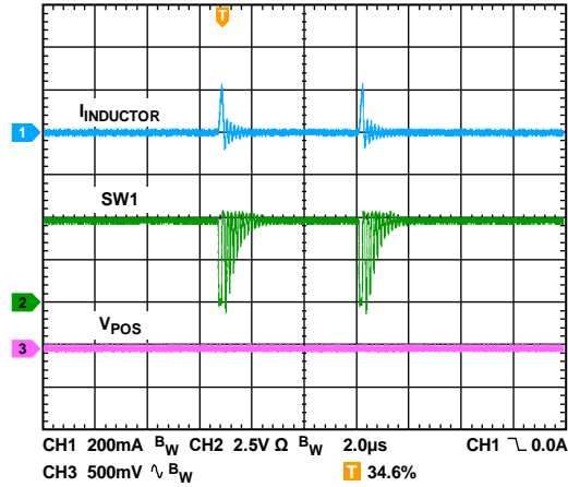
Figure 34. Boost Regulator Skip Mode Operation Showing Inductor Current ( I_{INDUCTOR} ), Switch Node Voltage, and Output Ripple, V_{IN} = 5\text{ V} , V_{POS} = 15\text{ V} , I_{LOAD1} = 4\text{ mA} , f_{SW} = 2.4\text{ MHz} , T_A = 25^\circ\text{C}
