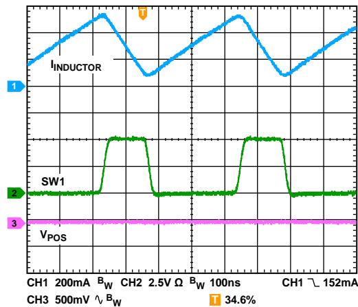
Figure 36. Boost Regulator Continuous Conduction Mode Operation Showing Inductor Current ( I_{INDUCTOR} ), Switch Node Voltage, and Output Ripple, V_{IN} = 5\text{ V} , V_{POS} = 15\text{ V} , I_{LOAD1} = 90\text{ mA} , f_{SW} = 2.4\text{ MHz} , T_A = 25^\circ\text{C}
