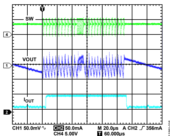
Figure 25. BUCK1 Response to Load Transient, I_{OUT1} from 1\text{ mA} to 50\text{ mA} , V_{OUT1} = 3.3\text{ V} , Auto PWM/PSM Mode
