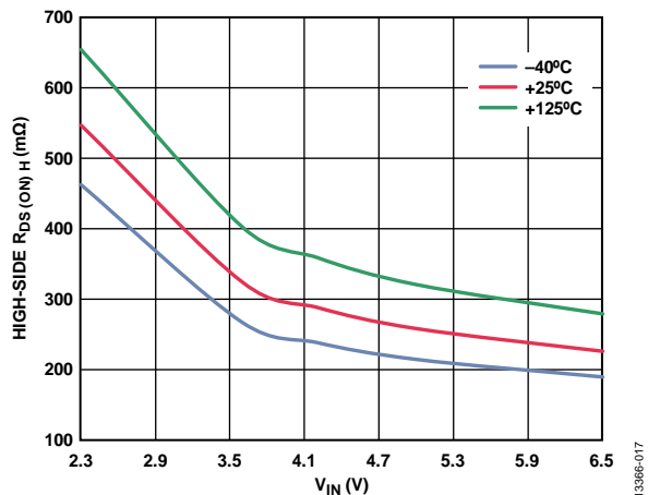
Figure 17. High-Side R_{DS(ON)} vs. V_{IN}
