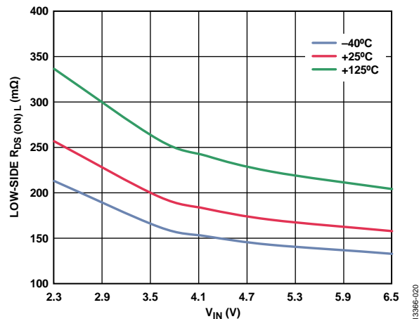
Figure 20. Low-Side R_{DS(ON)} vs. V_{IN}
