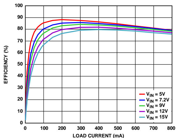
Figure 10. Channel 1 PWM Efficiency vs. Load Current, V_{OUT1} = 1.8\text{ V}
