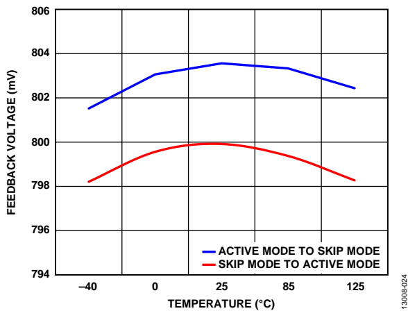
Figure 24. Channel 1 Feedback Voltage of PSM Mode vs. Temperature
