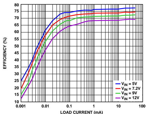
Figure 12. Channel 2 Hysteresis Efficiency vs. Load Current, V_{OUT2} = 1.2\text{ V}
