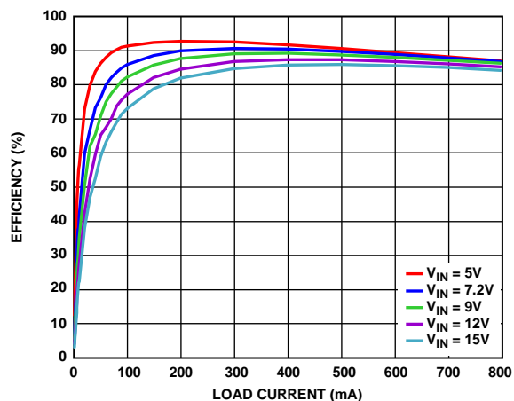
Figure 11. Channel 1 PWM Efficiency vs. Load Current, V_{OUT1} = 3.3\text{ V}
