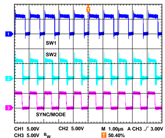
Figure 44. Synchronization to 1 MHz
