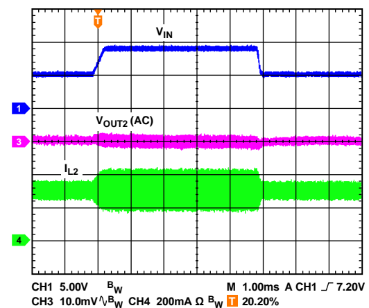
Figure 45. Channel 2 Line Transient in PWM Mode
