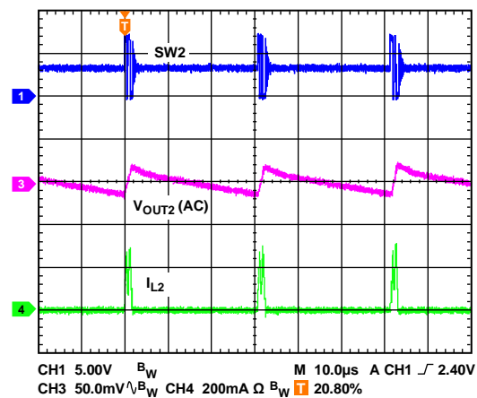
Figure 43. Channel 2 Output Ripple of Hysteresis Mode
