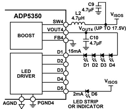
Figure 54. Four LEDs in Series (15 mA Each) for Grouped Backlight Connected to D1, and One LED Strip or Indicator (2 mA) in D5 with Connection to V_{ISOS} Rail
