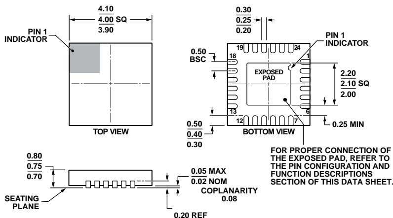
Figure 21. 24-Lead Lead Frame Chip Scale Package [LFCSP_WQ] 4 mm × 4 mm Body, Very Very Thin Quad (CP-24-10)
