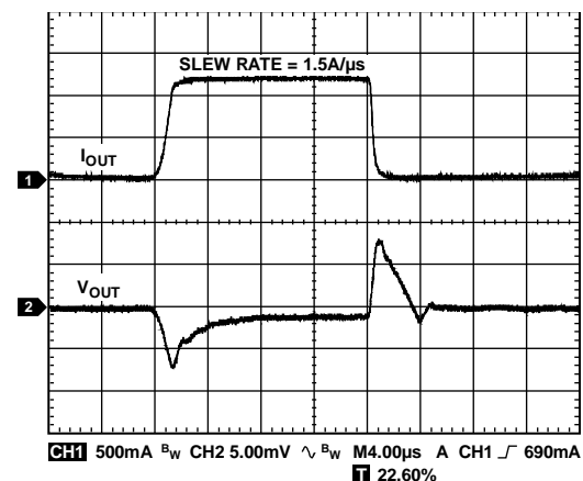
Figure 34. Load Transient Response, I_{\text{LOAD}} = 100\text{ mA} to 1.2\text{ A} , V_{\text{OUT}} = 3.3\text{ V} , V_{\text{IN}} = 4.0\text{ V} , C_{\text{OUT}} = 22\mu\text{F} , Channel 1 = I_{\text{OUT}} , Channel 2 = V_{\text{OUT}}
