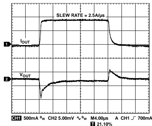
Figure 33. Load Transient Response, I_{\text{LOAD}} = 100\text{ mA} to 1.2\text{ A} , V_{\text{OUT}} = 3.3\text{ V} , V_{\text{IN}} = 4.0\text{ V} , Channel 1 = I_{\text{OUT}} , Channel 2 = V_{\text{OUT}}
