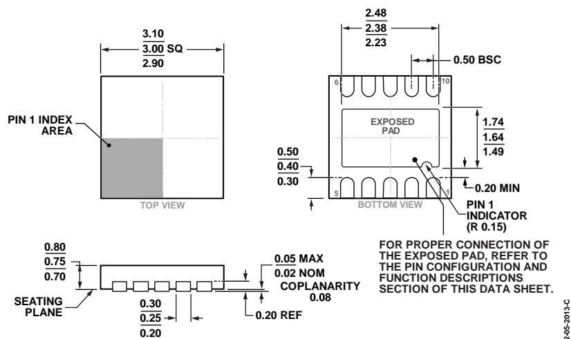
Figure 64. 10-Lead Lead Frame Chip Scale Package [LFCSP] 3 mm × 3 mm Body and 0.75 mm Package Height (CP-10-9)
