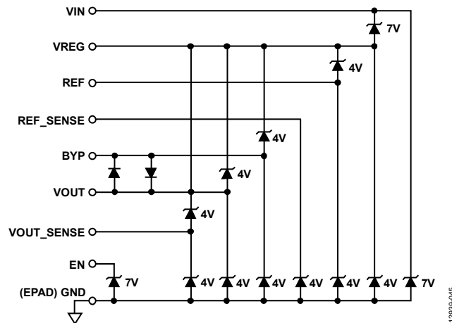
Figure 43. Simplified ESD Protection Block Diagram
