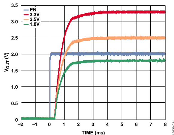
Figure 39. V_{OUT} Start-Up Time After V_{EN} Rising at Various Output Voltages, V_{IN} = 5.0 V, C_{BYP} = 1 \mu F
