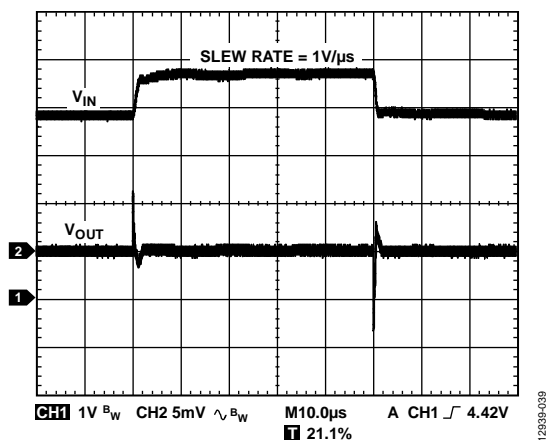
Figure 37. Line Transient Response, 1 V Input Step, I_{LOAD} = 2 A, V_{OUT} = 3.3 V, V_{IN} = 3.8 V, Channel 1 = V_{IN} , Channel 2 = V_{OUT}
