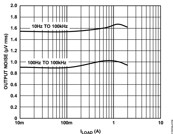
Figure 28. RMS Output Noise vs. Load Current ( I_{LOAD} )
