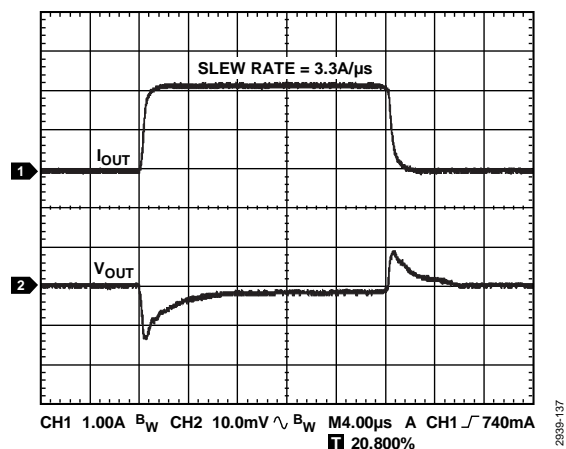
Figure 35. Load Transient Response, I_{LOAD} = 100 mA to 2 A, V_{OUT} = 1.8 V, V_{IN} = 2.5 V, Channel 1 = I_{OUT} , Channel 2 = V_{OUT}
