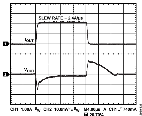
Figure 36. Load Transient Response, I_{LOAD} = 100 mA to 2 A, V_{OUT} = 1.8 V, V_{IN} = 2.5 V, C_{OUT} = 22 \mu F, Channel 1 = I_{OUT} , Channel 2 = V_{OUT}
