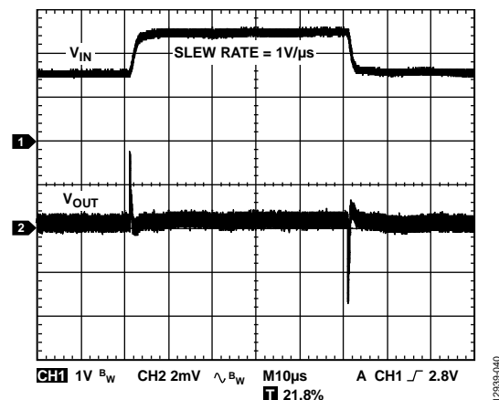
Figure 38. Line Transient Response, 1 V Input Step, I_{LOAD} = 2 A, V_{OUT} = 1.8 V, V_{IN} = 2.5 V, Channel 1 = V_{IN} , Channel 2 = V_{OUT}
