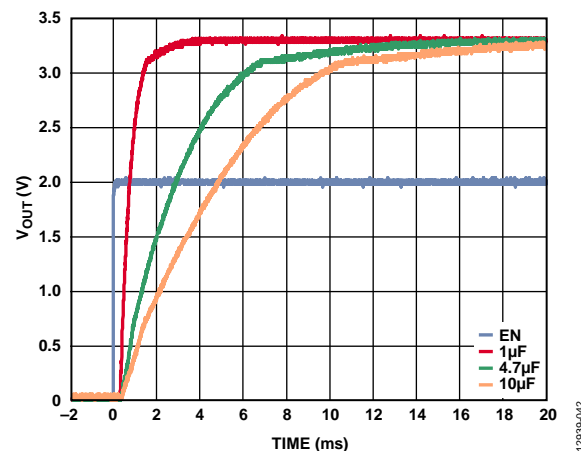
Figure 40. V_{OUT} Start-Up Time Behavior at Various Values of C_{BYP} , V_{OUT} = 3.3 V
