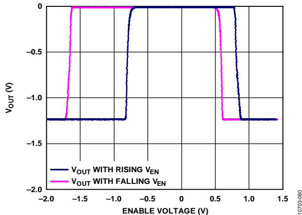
Figure 82. Typical EN Pin Operation
