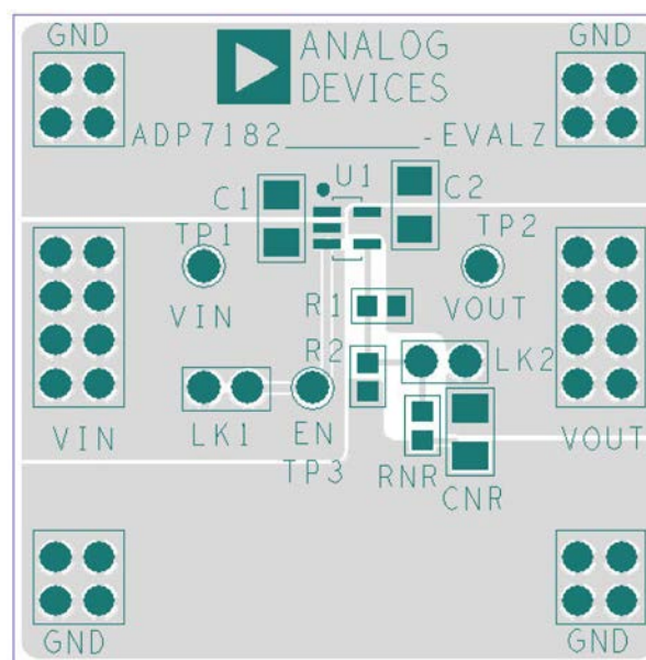
Figure 103. Example of the 5-Lead TSOT PCB Layout
