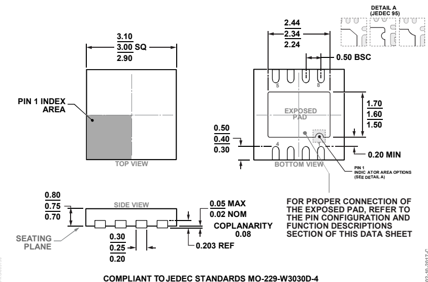
Figure 105. 8-Lead Lead Frame Chip Scale Package [LFCSP] 3 mm × 3 mm Body and 0.75 Package Height (CP-8-11) Dimensions shown in millimeters
