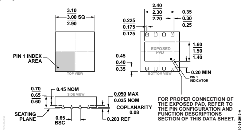
Figure 18. 8-Lead Lead Frame Chip Scale Package [LFCSP] 3 mm × 3 mm Body and 0.65 mm Package Height (CP-8-22)
