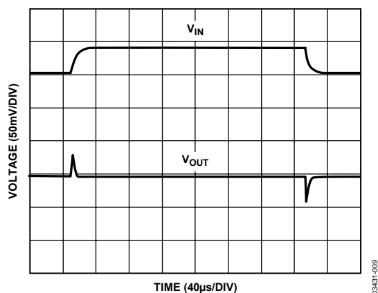
Figure 9. Line Transient Response, C_{BYPASS} = 0\text{ μF}
