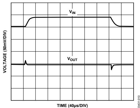
Figure 10. Line Transient Response, C_{BYPASS} = 0.1\text{ μF}
