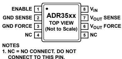
Figure 2. Pin Configuration
