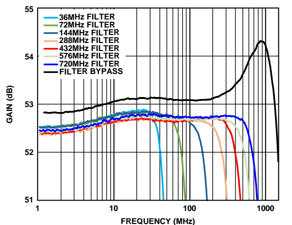
Figure 11. Gain vs. Frequency over all Bandwidth Settings; VGN1 = VGN2 = 1.5 V (Logarithmic)
