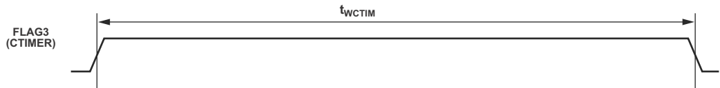
Figure 10. Core Timer
