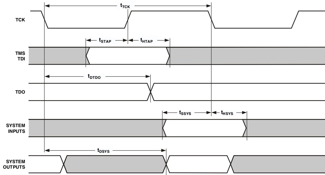
Figure 17. JTAG Port Timing
