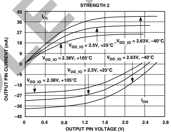
Figure 26. Typical Drive Currents at Strength 2
