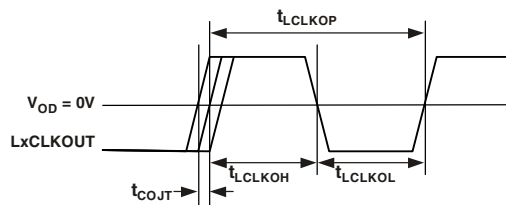
Figure 16. Link Ports—Output Clock
