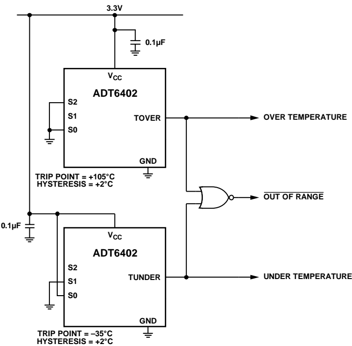
Figure 17. Temperature Window Alarms
