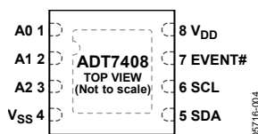
Figure 4. Pin Configuration
