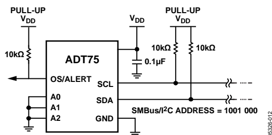
Figure 13. Typical SMBus/I 2 C Interface Connection
