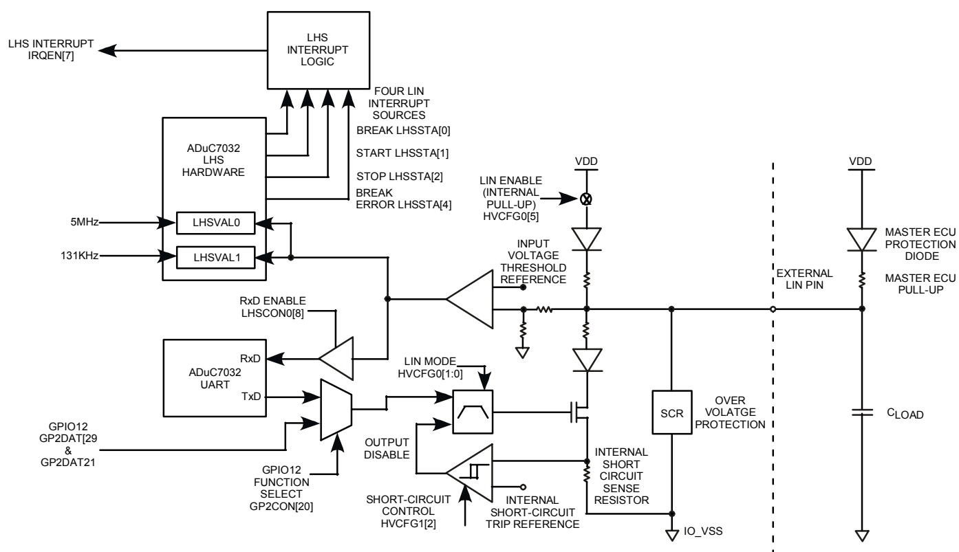
Figure 38: LIN I/O, Block Diagram
