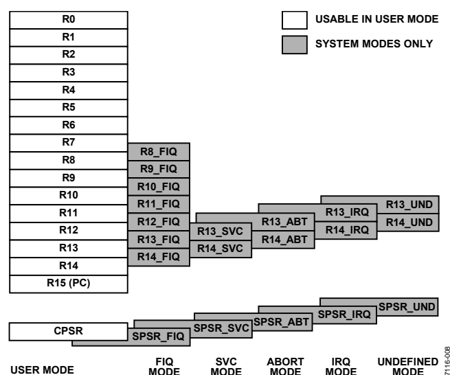
Figure 11. Register Organization
