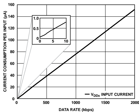
Figure 13. Current Consumption per Input vs. Data Rate for 2.5 V, EN_x = \text{High Operation}
