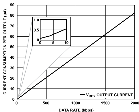
Figure 14. Current Consumption per Output vs. Data Rate for 2.5 V, EN_x = \text{High Operation}
