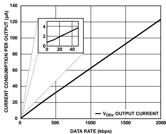
Figure 12. Current Consumption per Output vs. Data Rate for 3.3 V, EN_x = \text{Low Operation}
