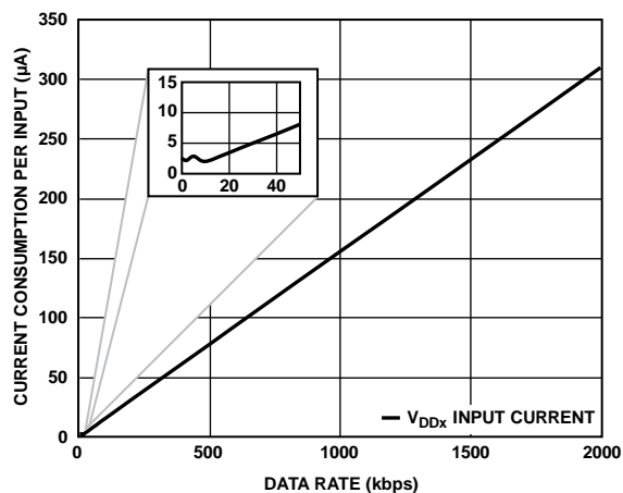
Figure 9. Current Consumption per Input vs. Data Rate for 2.5 V, EN_x = \text{Low Operation}
