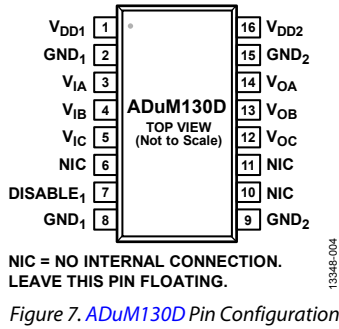
Figure 7. ADuM130D Pin Configuration
