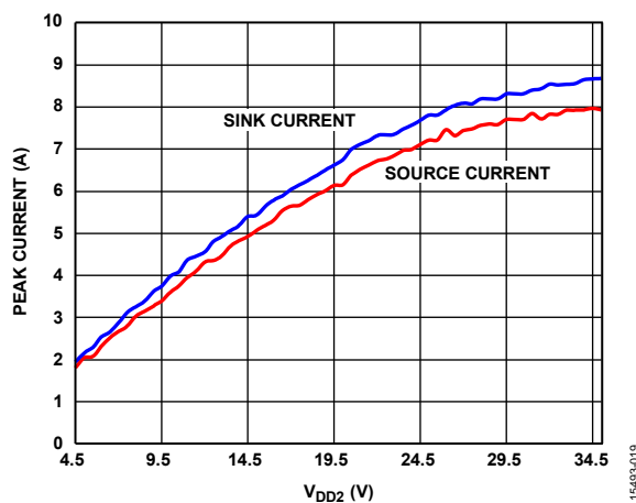
Figure 19. Peak Current vs. V_{DD2} , 2 \Omega Resistor
