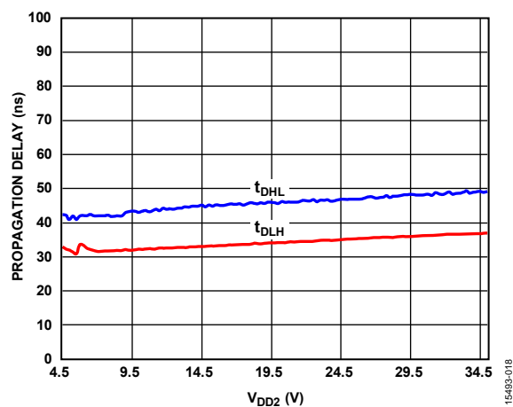
Figure 18. ADuM4120-1 Propagation Delay vs. V_{DD2} , 2 nF Load
