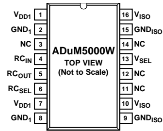
Figure 3. Pin Configuration
