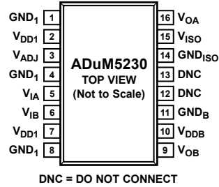
Figure 3. Pin Configuration
