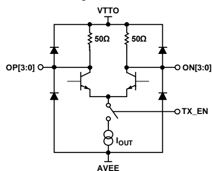
Figure 26. High Speed Output Simplified Schematic
