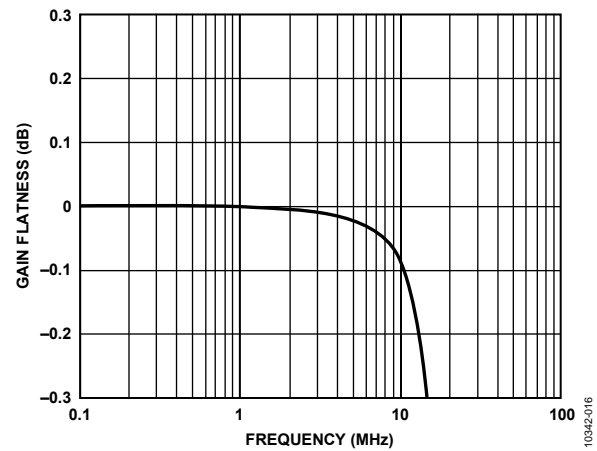
Figure 11. Large Signal Gain Flatness, V_{OUT} = 2\text{ V p-p}
