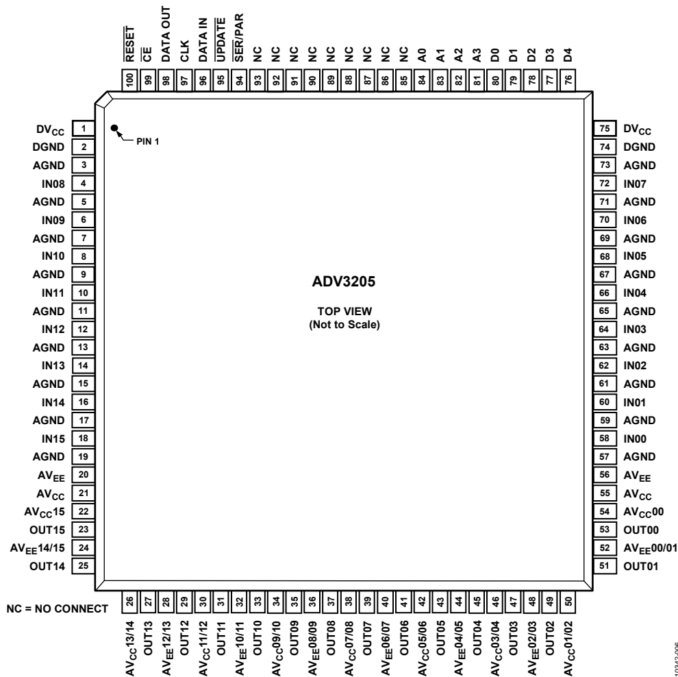
Figure 5. Pin Configuration
