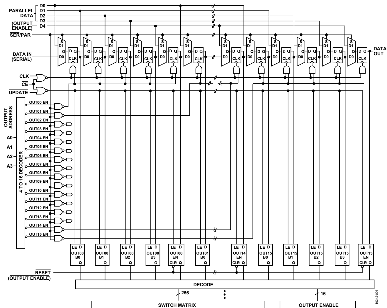
Figure 6. Logic Diagram
