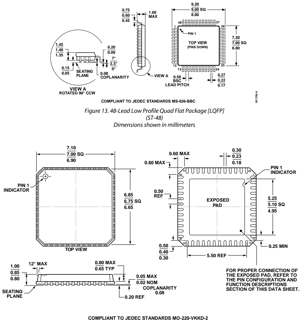
Figure 14. 48-Lead Lead Frame Chip Scale Package [LFCSP] 7 mm × 7 mm Body and 0.85 mm Package Height (CP-48-1) Dimensions shown in millimeters
