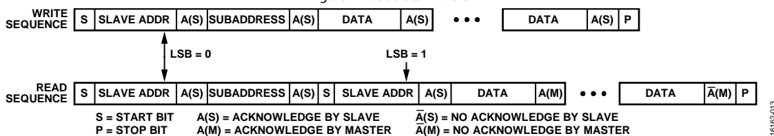
Figure 13. Read and Write Sequence
