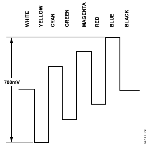
Figure 123. Pb Levels—PAL
