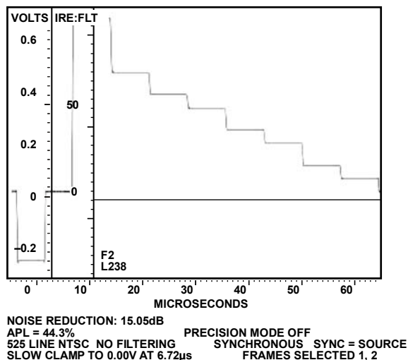
Figure 133. NTSC Luma
