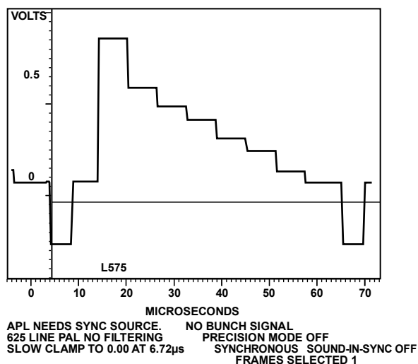
Figure 136. PAL Luma
