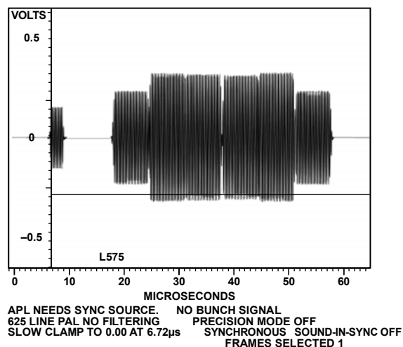
Figure 137. PAL Chroma
