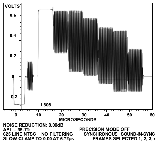
Figure 135. PAL Color Bars (75%)
