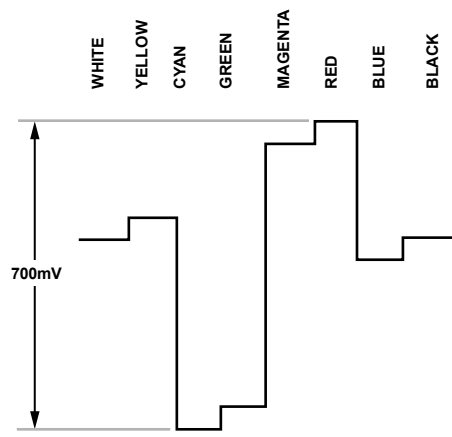
Figure 122. Pr Levels—PAL
