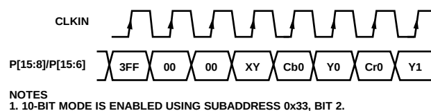
Figure 61. ED (at 54 MHz) Input Sequence (EAV/SAV)
