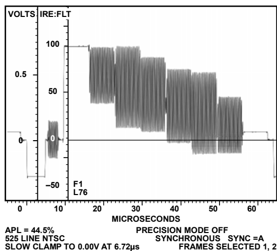
Figure 132. NTSC Color Bars (75%)
