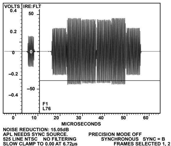
Figure 134. NTSC Chroma
