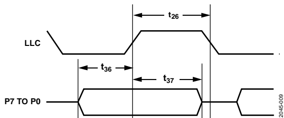
Figure 9. 8-Bit Digital Pixel Video Output, SDR Video Data Timing
