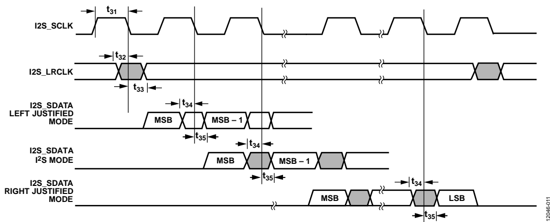
Figure 11. I²S Timing
