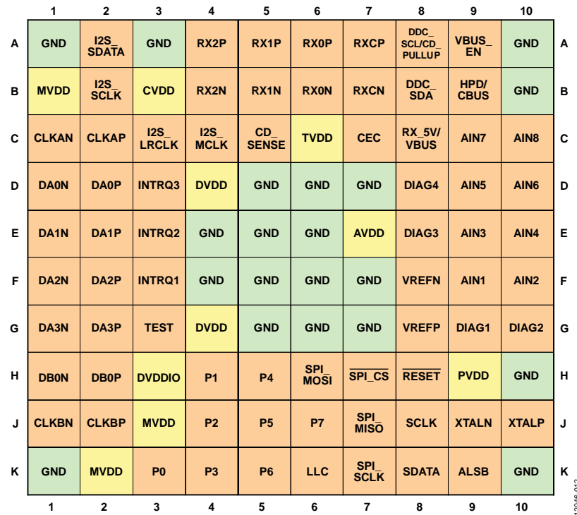
Figure 12. Pin Configuration
