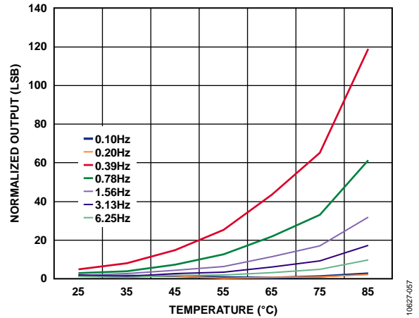
Figure 45. Typical Y-Axis Output vs. Temperature at Lower Data Rates, Normalized to 100 Hz Output Data Rate, V_S = 2.5\text{ V}
