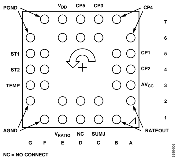
Figure 3. Pin Configuration
