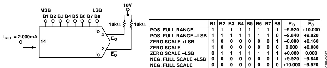
Figure 26. Basic Bipolar Output Operation
