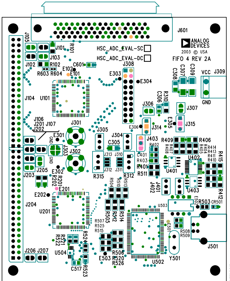
Figure 34. Assembly—Primary Side
