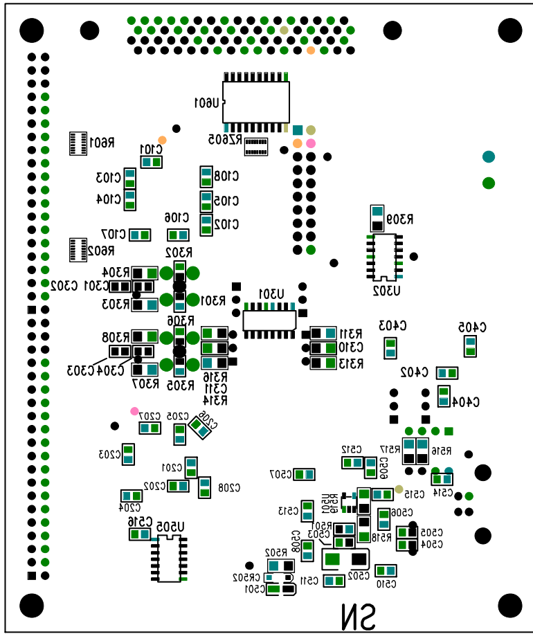
Figure 35. Assembly—Secondary Side
