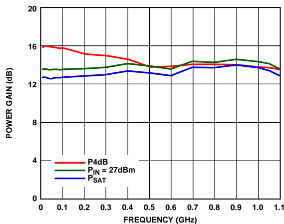
Figure 20. Power Gain vs. Frequency
