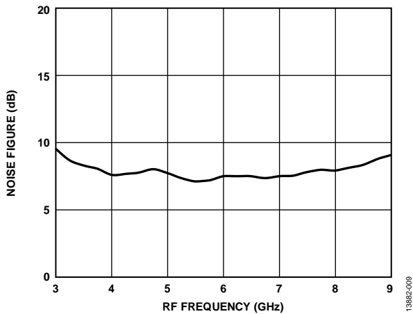
Figure 9. Noise Figure vs. RF Frequency at 25^\circ\text{C} , LO = 15 dBm
