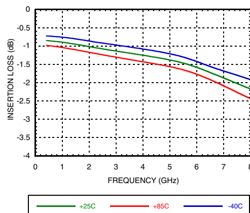
Normalized Attenuation
