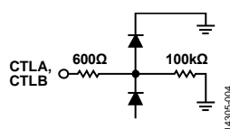
Figure 4. CTLA and CTLB Interface Schematic
