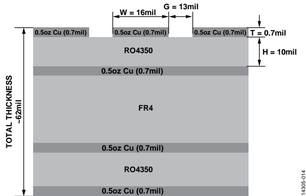
Figure 14. EV1HMC344ALP3 Evaluation Board (Cross Sectional View)
