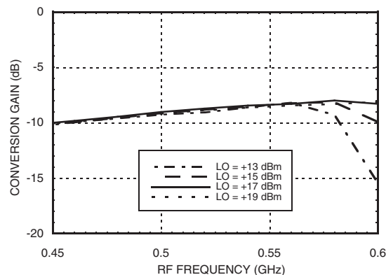
Upconverter Conversion Gain vs. LO Drive
