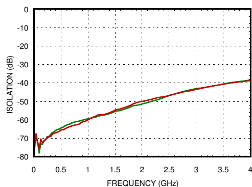
Isolation Between Ports RF1 and RF2
