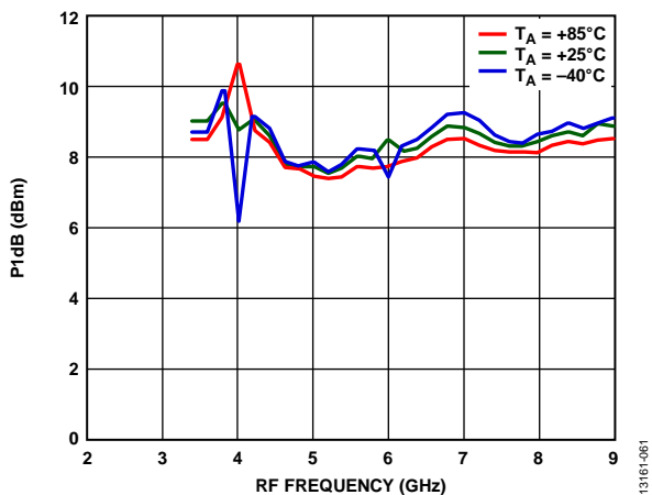
Figure 65. Input P1dB vs. RF Frequency at Various Temperatures, LO Drive = 15 dBm
