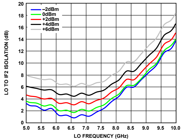
Figure 83. LO to IF2 Isolation vs. LO Frequency over LO Powers, T A = 25°C, Voltage Control = -4 V
