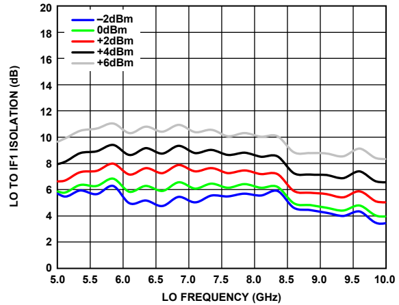
Figure 82. LO to IF1 Isolation vs. LO Frequency over LO Powers, T A = 25°C, Voltage Control = -4 V
