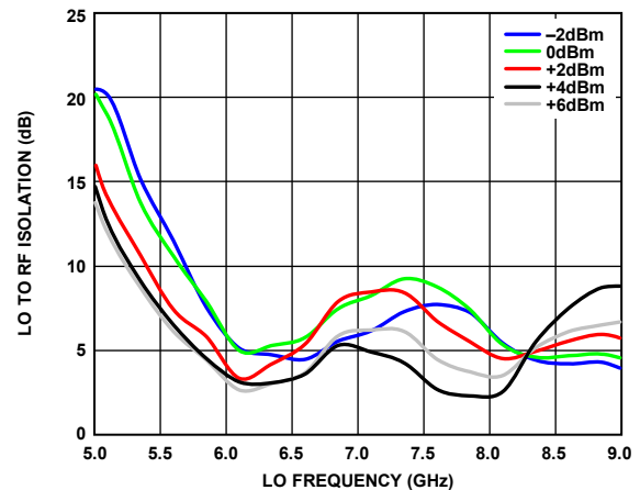
Figure 84. LO to RF Isolation vs. LO Frequency over LO Powers, T A = 25°C, Voltage Control = -4 V
