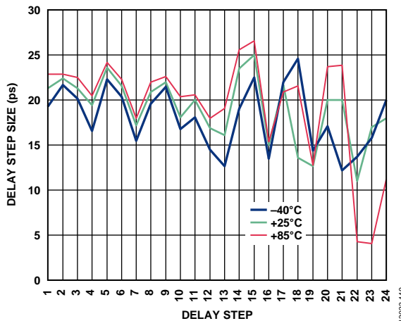
Figure 20. Analog Delay Step Size vs Delay Step over Temperature, LVPECL at 3072 MHz with Digital Delay = 0
