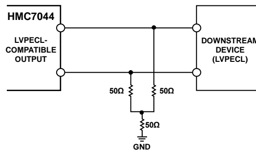
Figure 32. DC-Coupled LVPECL Output Driver
