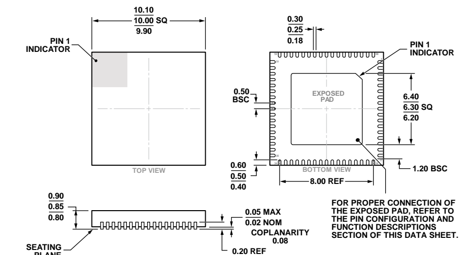
Figure 54. 68-Lead Lead Frame Chip Scale Package [LFCSP_VQ] 10 mm x 10 mm Body, Very Thin Quad (HCP-68-1) Dimensions shown in millimeters
