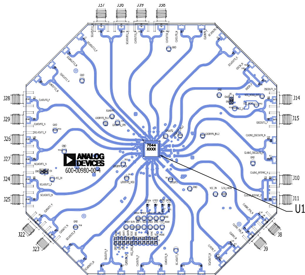
Figure 52. Evaluation PCB Layout, Top Side
