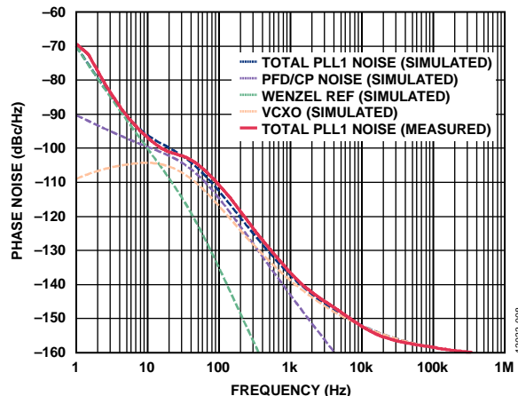
Figure 6. Closed-Loop Phase Noise at 122.88 MHz, PLL1 Measurement vs. Simulated, Clean Reference Source, ~70 Hz Loop Bandwidth 80° Phase Margin
