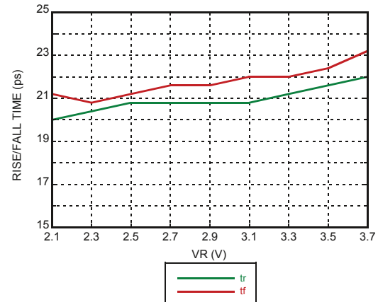
Rise / Fall Time vs. VR [1][2]
