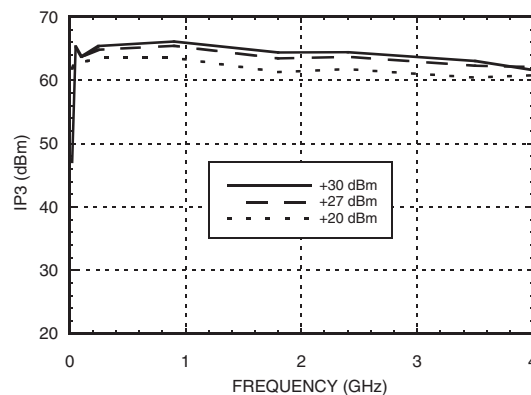
Input IP3 vs. Tone Power @ Vdd = +8V
